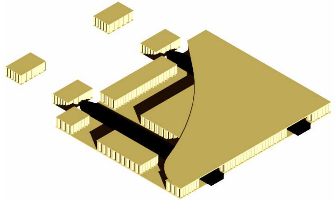
4-WAY FORKLIFT ENTRY ILLUSTRATION (Forks "Knock-Out" honeycomb blocks)
