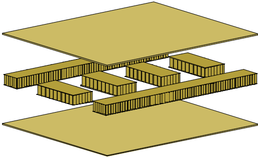
CONSTRUCTION ILLUSTRATION (48" x 40" pallet shown)
